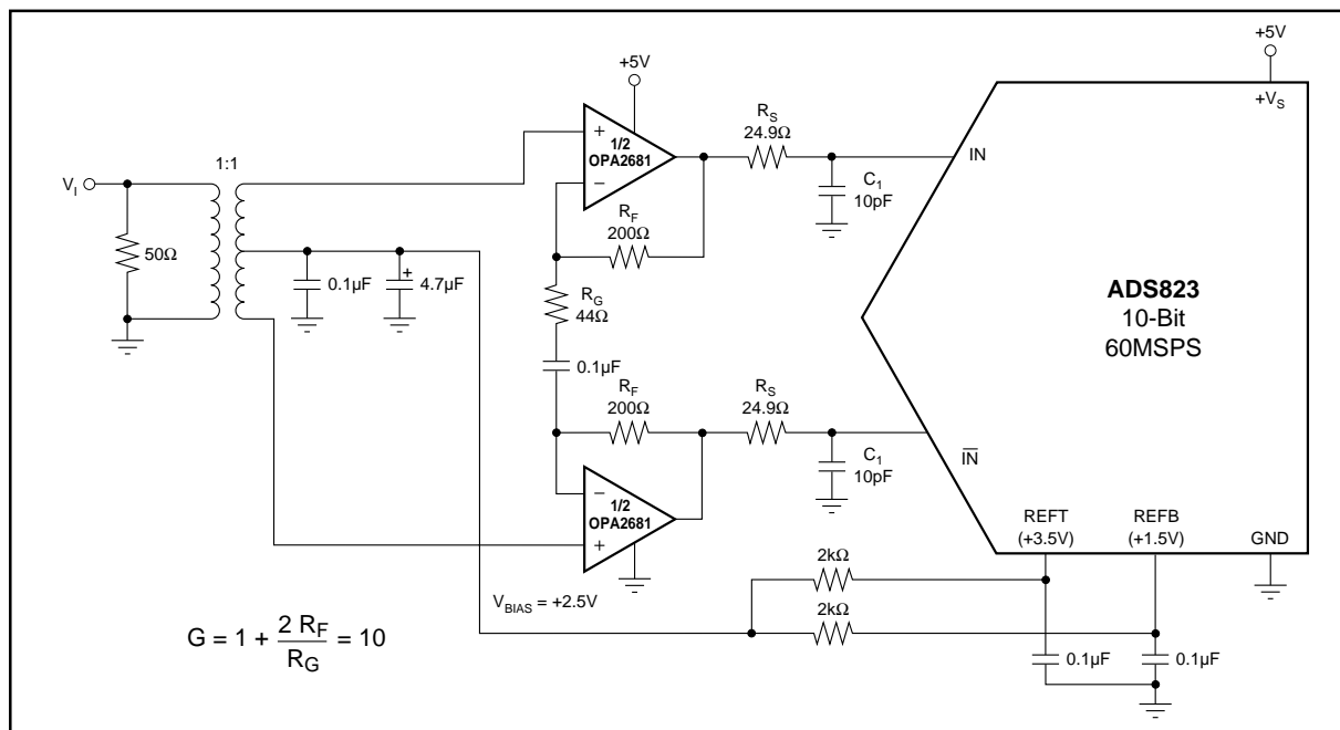
FIGURE 3. Wideband, Single Supply, Differential ADC Driver.
