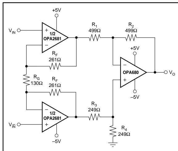
FIGURE 6. Wideband, 3-Op Amp Instrumentation Diff. Amp.
