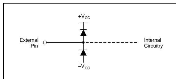
FIGURE 13. Internal ESD Protection.
