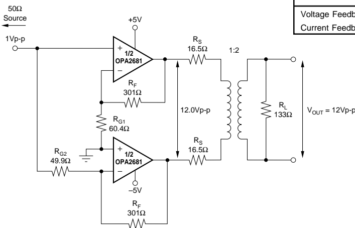
High Power Twisted Pair Driver
