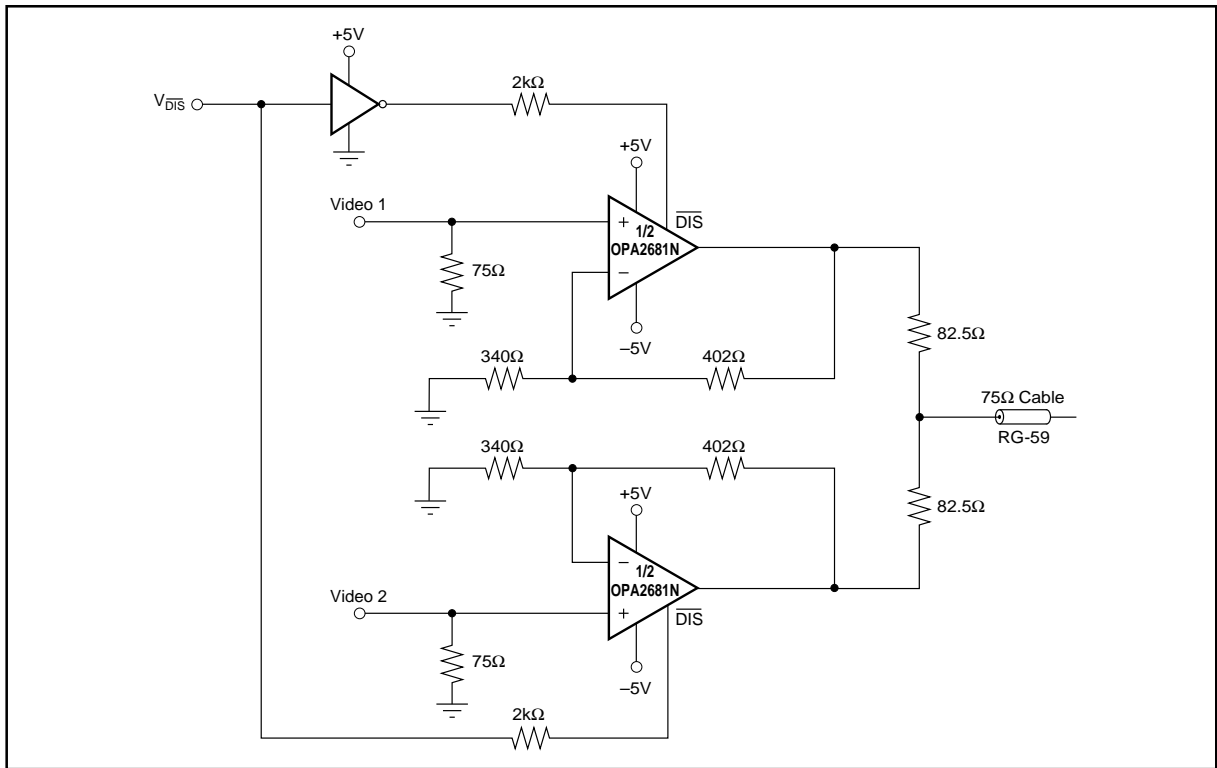
FIGURE 4. Two-Channel Video Multiplexer.
