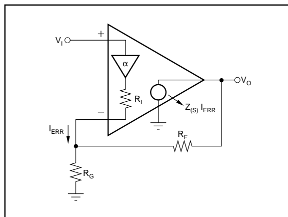
FIGURE 7. Current Feedback Transfer Function Analysis Circuit.
