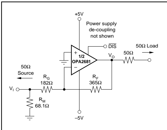
FIGURE 9. Inverting Gain of -2 with Impedance Matching.
