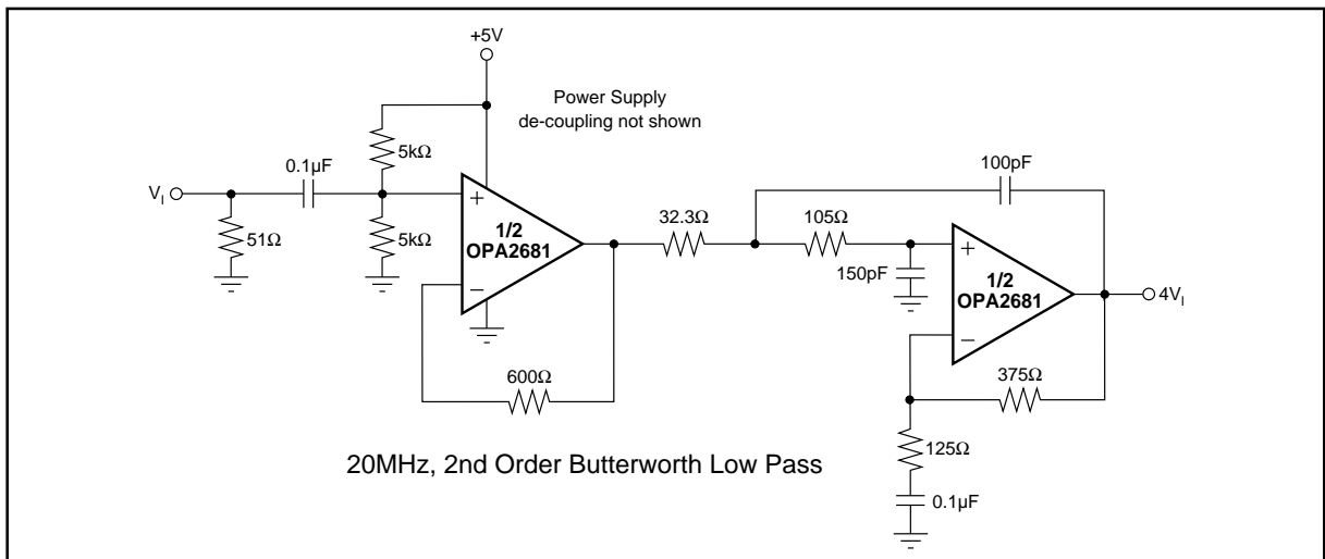
FIGURE 5. Buffered, Single Supply Active Filter.
