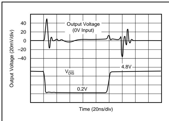
FIGURE 12. Disable/Enable Glitch.
