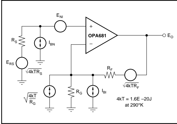
FIGURE 10. Op Amp Noise Analysis Model.
